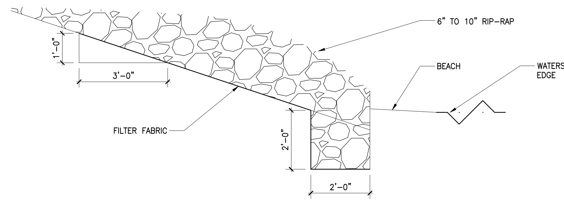
1 SECTION THROUGH SHORELINE
