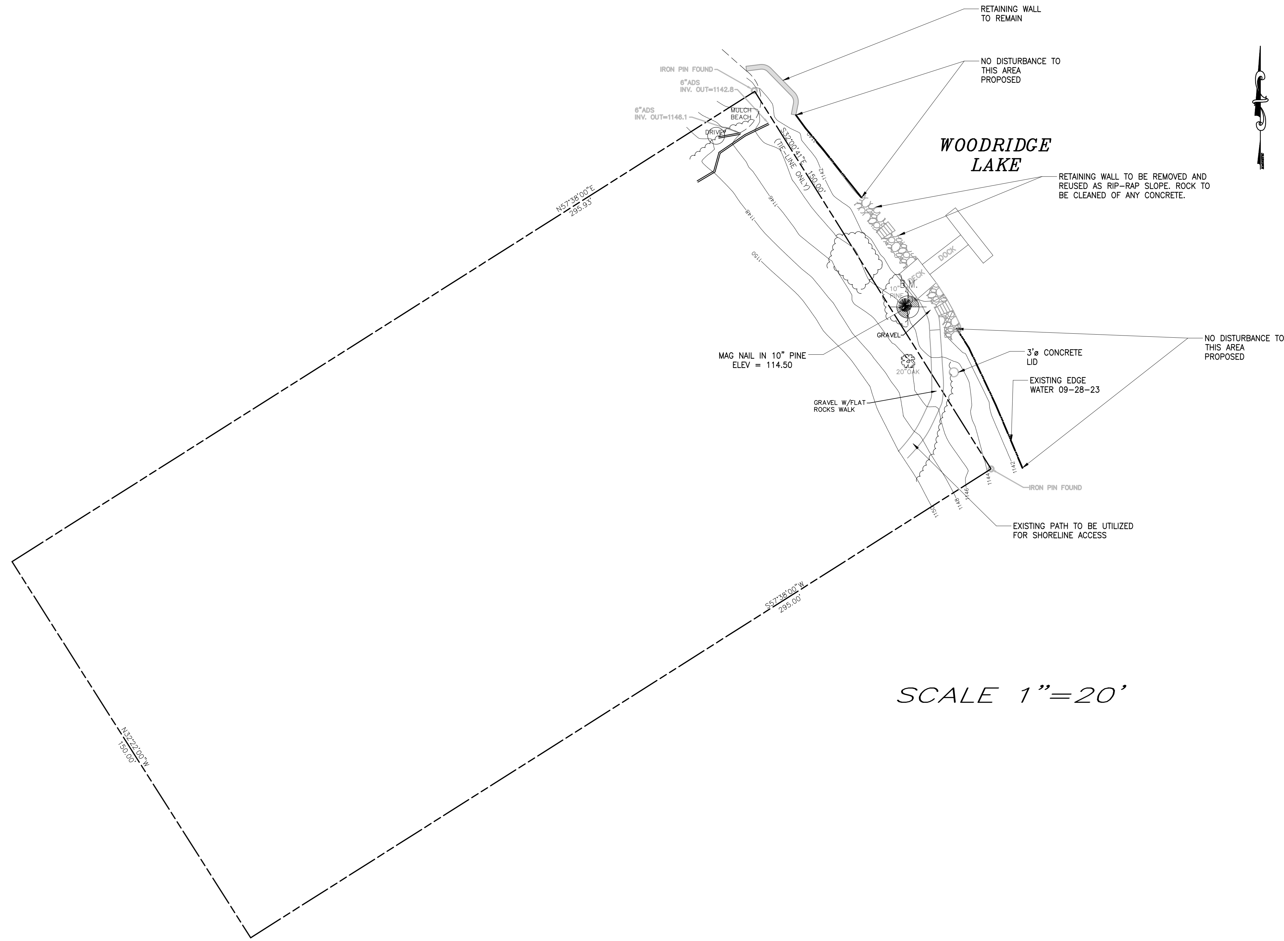
2 SITE DEVELOPMENT PLAN
